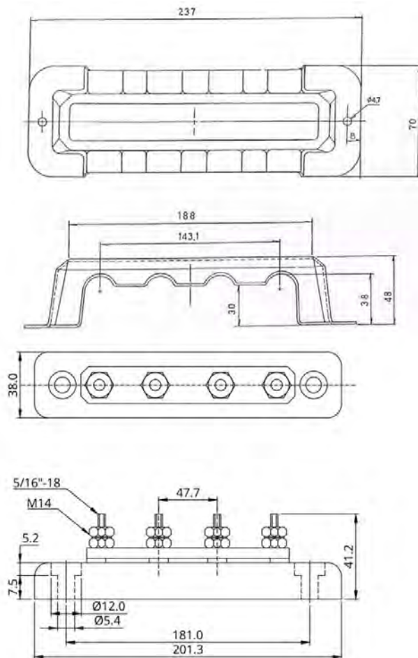
Busbar 250 A with 4 stud terminals and cover
