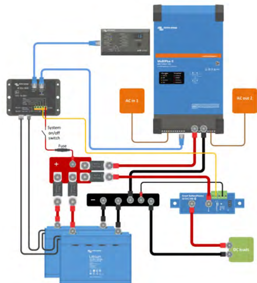
Figure 5: System with MultiPlus-II and DC loads
