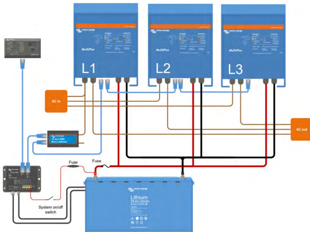
Figure 8: System example for a boat or vehicle with a three phase inverter/charger configuration (DC fuses not shown, except for the Li-ion battery fuse) Note 1: the AC Detector is installed in the leader only. Note 2: the BMS is connected to the battery minus by the UTP cable between the BMS and the inverter/charger. Therefore, in order to prevent ground loops, do not wire the BMS minus connector.
