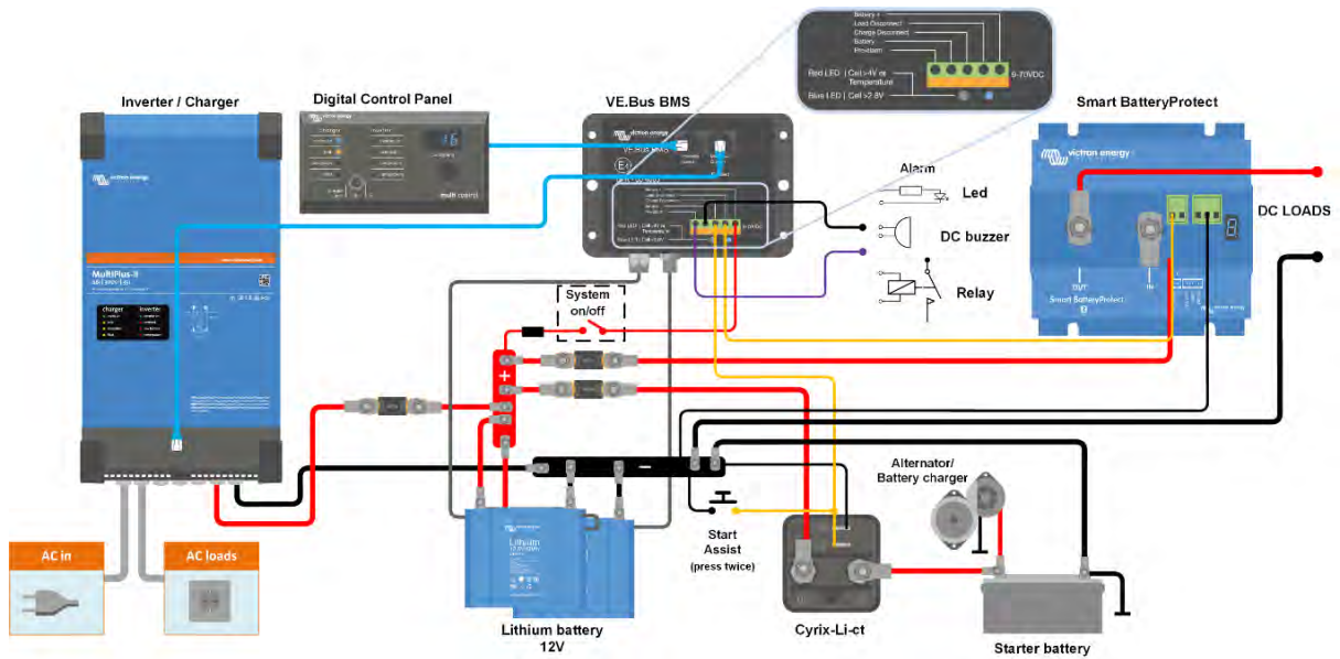
Figure 7: System for a boat or vehicle with a MultiPlus-II inverter/charger Note: the BMS is connected to the battery minus by the UTP cable between the BMS and the inverter/charger. Therefore, in order to prevent ground loops, do not wire the BMS minus connector.
